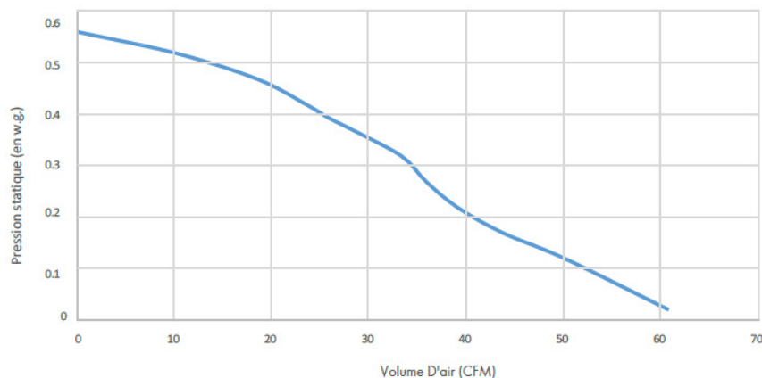
COURBE DE PERFORMANCE HVI
